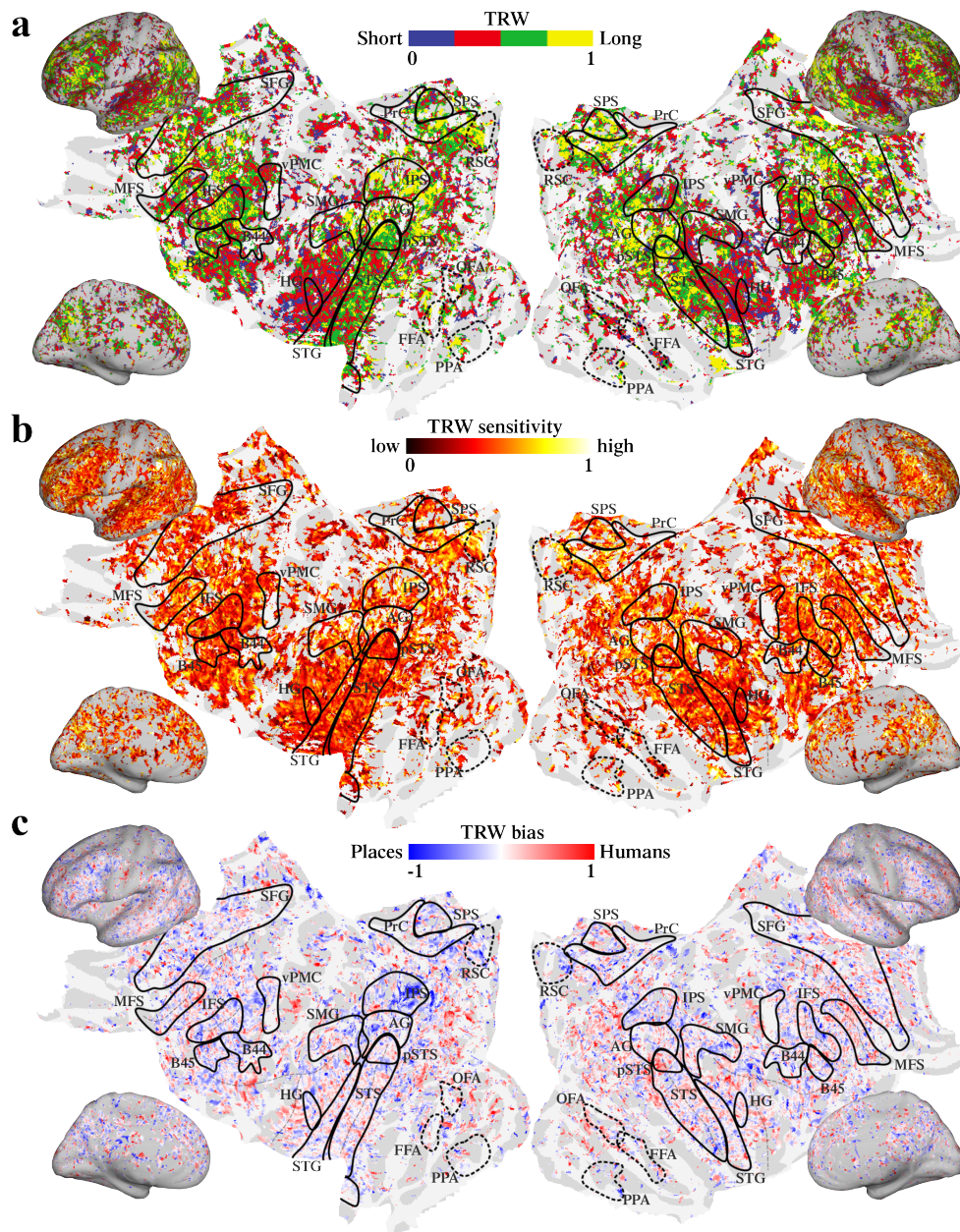
Figure 1: Attentional modulation of TRW across cortex. HG, Heschl's gyrus; STS, superior temporal sulcus; SMG, superior middle gyrus; vPMC, ventral premotor cortex; BA44/BA45, Brodmann area 44/45; AG, angular gyrus; IPS, intraparietal sulcus; SPS, subparietal sulcus; PrC, precuneus; IFS, inferior frontal sulcus; MFS, middle frontal sulcus; SFG, superior frontal gyrus; FFA, fusiform face area; OFA, occipital face area; PPA, parahippocampal place area; RSC, retrosplenial cortex. Voxels for which the prediction score of the unscrambled model was lower than the average appear as gray curvature and were not included in the analyses. (a) Normalized TRW averaged across five subjects. TRW increases from early auditory areas toward higher auditory areas and parietal and prefrontal areas. (b) Attentional sensitivity of TRW averaged across five subjects. Attentional sensitivity of TRW is relatively low in early auditory areas and category-selective areas. (c) Attentional bias of TRW averaged across five subjects. TRW bias was not significant in early auditory areas in temporal cortex (bootstrap test, p > 0.05 ). However, bias is more prominent in higher cognitive areas in prefrontal cortex (BA45, IFS, MFS, SFG), inferior parietal cortex (IPS and AG), and category-selective areas.
