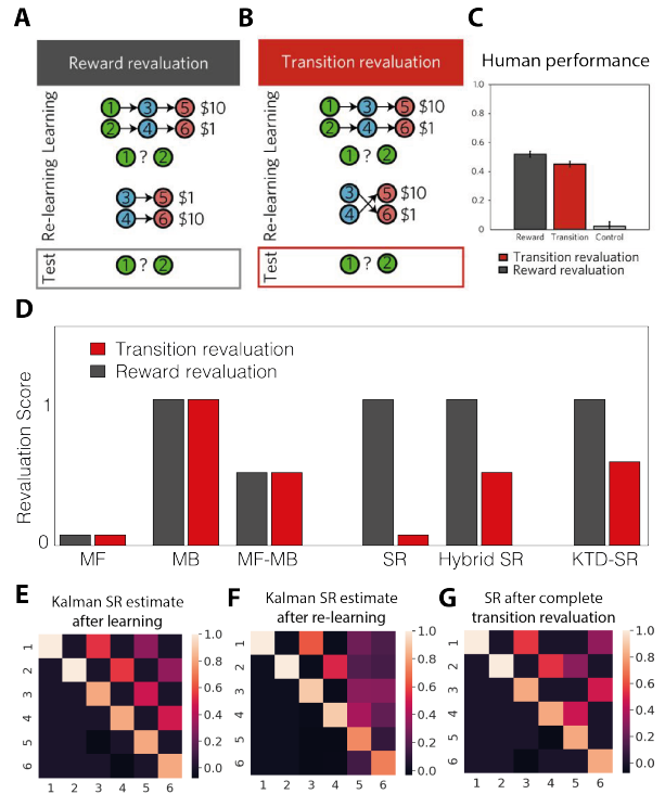
Figure 1: KTD SR performance on a transition and reward revaluation experiment. (A-B) Task structure for (A) reward revaluation and (B) transition revaluation experiments. (C) Human performance on transition and reward revaluation tasks. (D) Model predictions for classic model-free, model-based or a hybrid of model free and model-based algorithms, TD-SR, hybrid SR and KTD-SR. (E-G) The SR matrix estimated by KTD after (E) learning (phase 1), (F) re-learning (phase 2) and (G) after a hypothetical complete transition revaluation. Panels A–C reprinted with permission from Momennejad et al. (2017).
